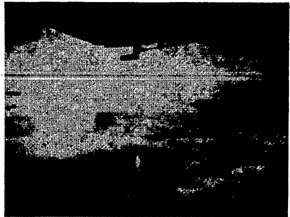
Figure 4.- Upper level of a stratified ice cloud, topped by loose water clouds(alto-stratus with alto-cumulus)
