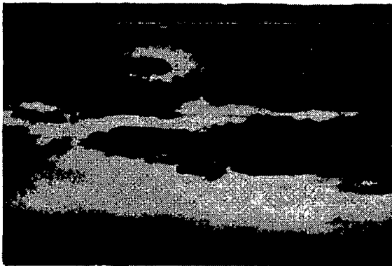
Figure 5.- Lower edge of a stratified ice cloud with water clouds beneath(nimbo-stratus with fracto-cumulus).
