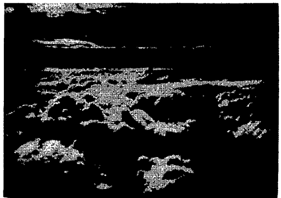
Figure 6.- Cumulous water clouds(cumulus, alto-cumulus)
