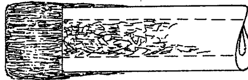
Ice on positive pitot head, showing opening partially closed and ice forming inside tube.
