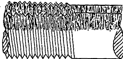
Formation on threaded end of streamline wire, note ice following contour of threads.
